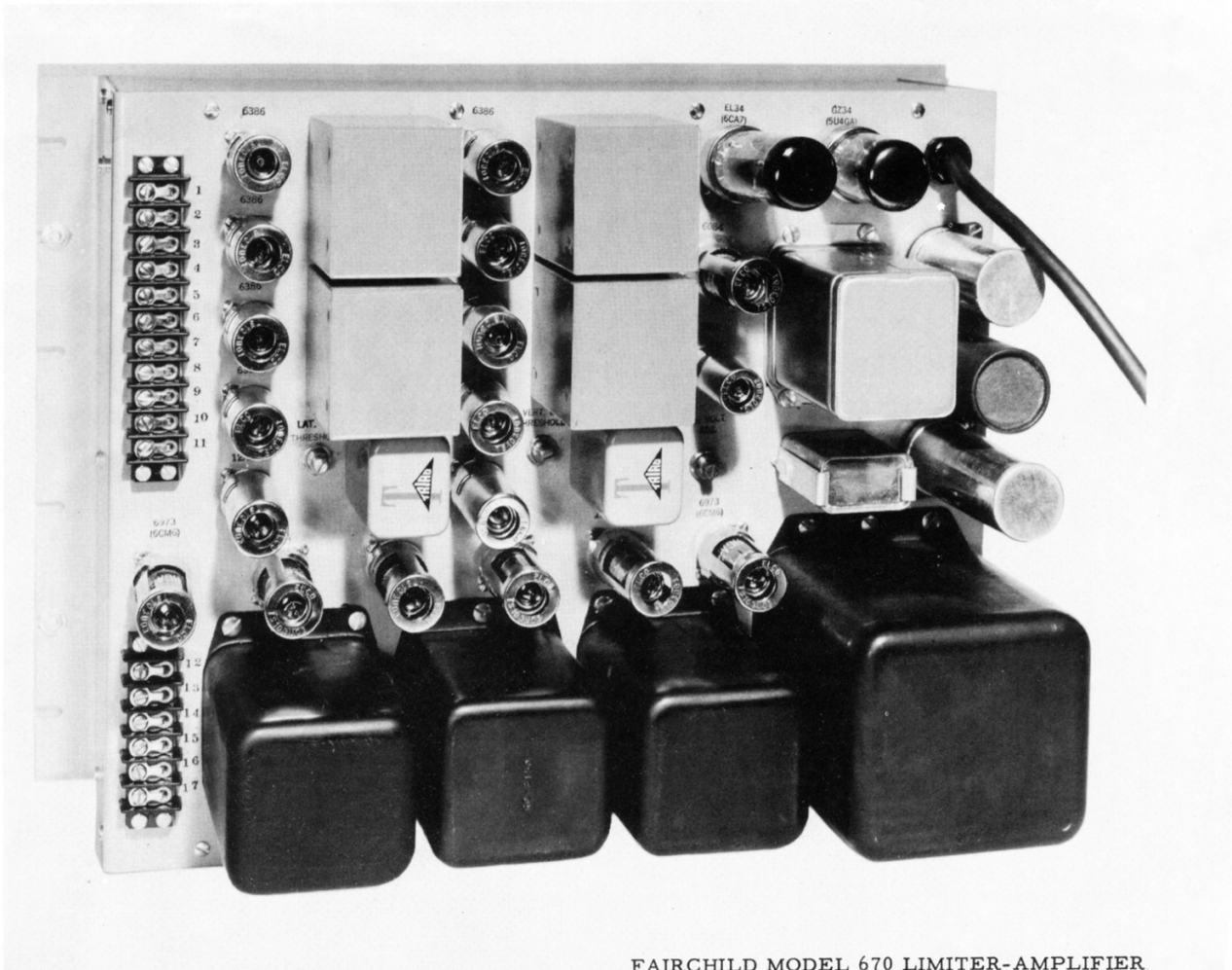
FAIRCHILD MODEL 670 LIMITER-AMPLIFIER TWO-CHANNEL FOR STEREO
